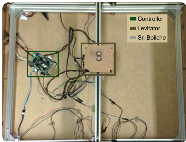
Figure 3: The hardware that is hidden below the playground. A microcontroller for controlling the stage. A levitator and the magnetic ball that is usually above the playground floor.
